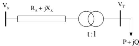
Figure 3: Model Thevenin Equivalent
